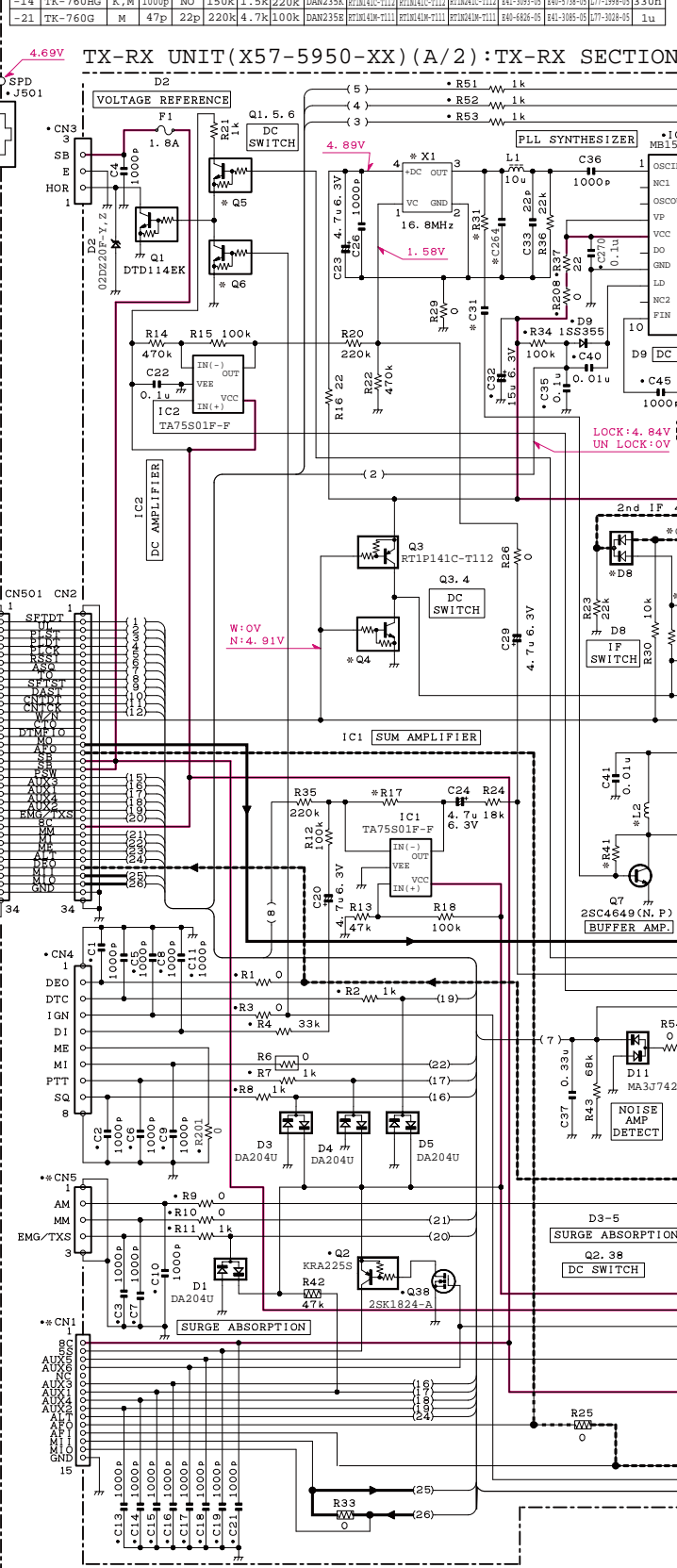
TX-RX UNIT(X57-5950-XX)(A/2):TX-RX SECTION
