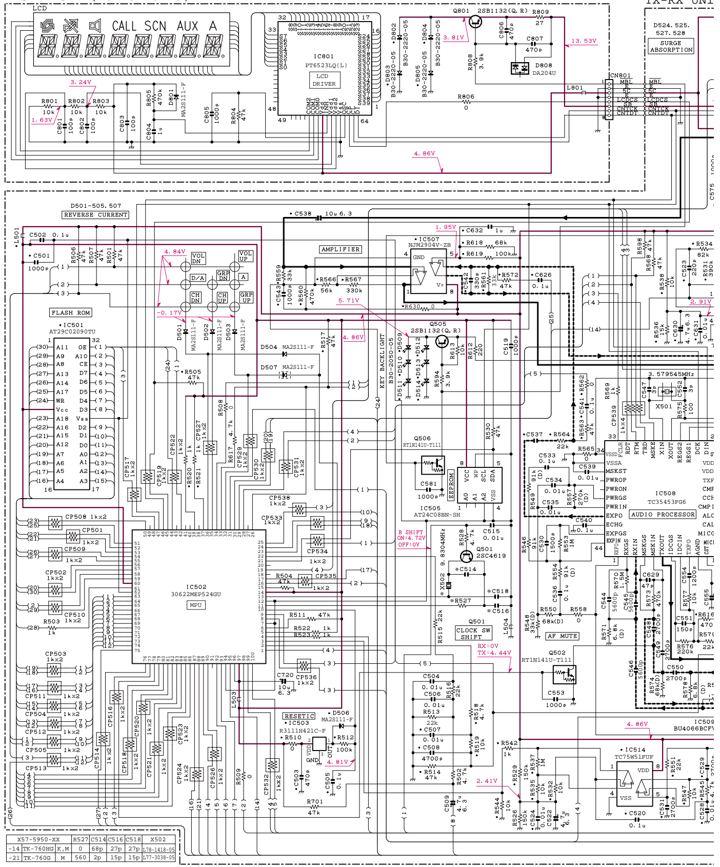
TX-RX UNIT (X57-5950-XX)(B2): CONTROL SECTION
